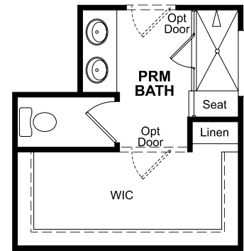
Opt Deluxe Primary Bathroom B
